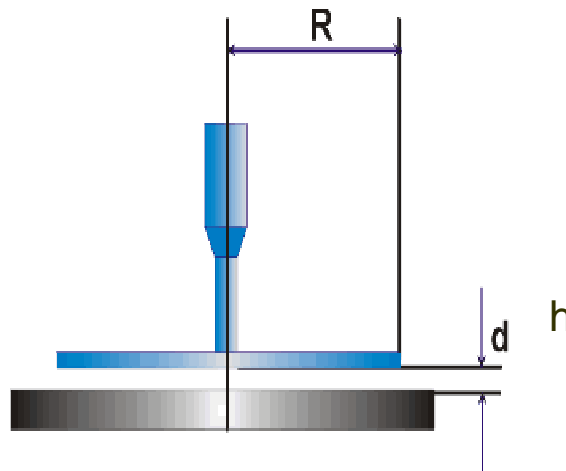
Figure 12 Schematic diagram of Parallel Plate Measuring System [104]
