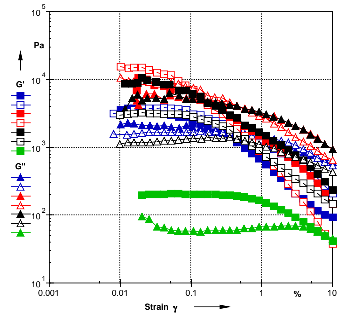
Figure 25 Comparison of amplitude sweep tests (CSD) of different waxes studied at 90°C
