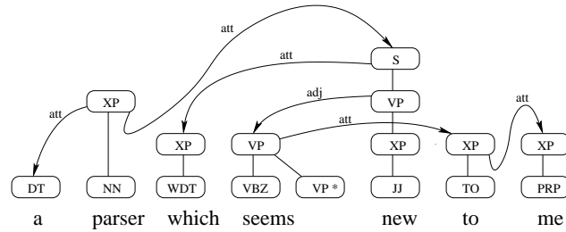
Figure 2. An example of an LTAG-spinal derivation
