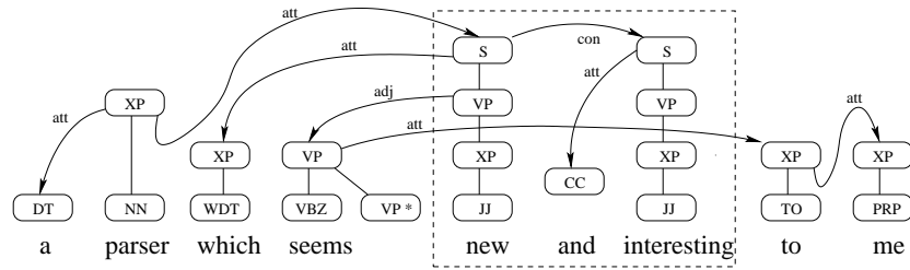
Figure 3. An example of conjoining in LTAG-spinal
