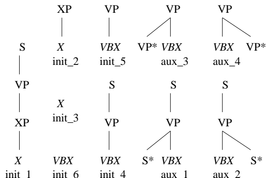
Figure 4. Types of normalized spinal e-trees
