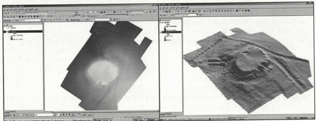
Figure 5 Hill-shade analysis draped over spline model, viewed in ArcScene
