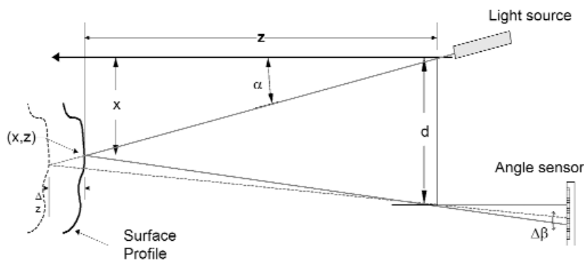
Figure 2a Principle of active triangulation: a triangulation-based laser probe
