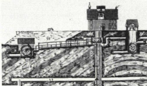
Figure 4 Two wheels are necessary, pumping water (l.) and transport of material, hoisting engine (r.) (Beyersdorf 1908)
