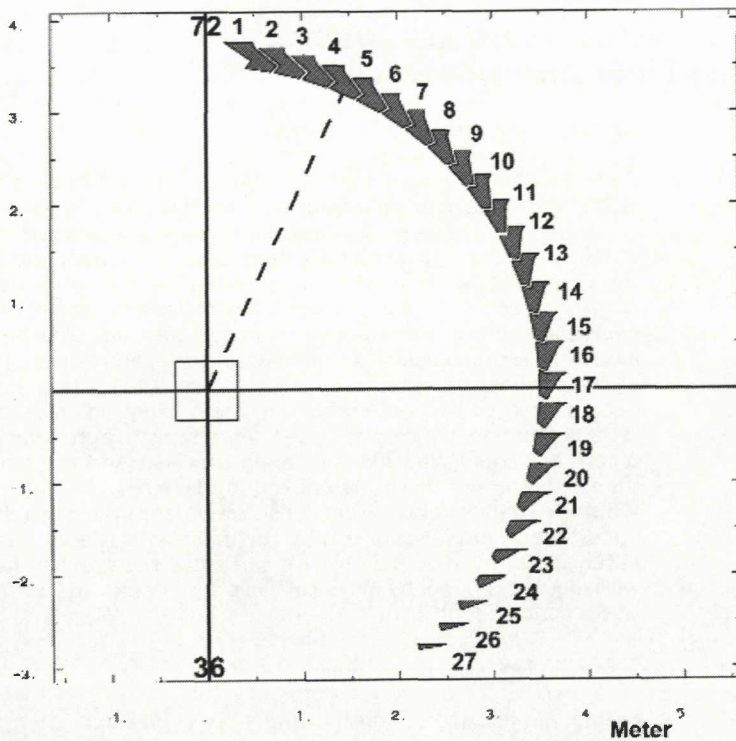
Figure 3 The effective content of the buckets decreases due to the motion of the wheel (FB)
