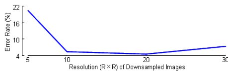
Figure 16. Error rate vs. Resolution. One-nearest-neighbor classification on Farsi dataset with four resolutions. Note that the error rate varies little when the resolution is greater than 10×10.
