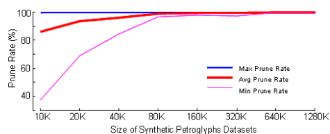
Figure 19. Pruning rate of our lower bound algorithm on eight synthetic petroglyphs datasets. For each dataset, maximal, average, and minimal rates are reported. Note: log scale is used in x axis.
