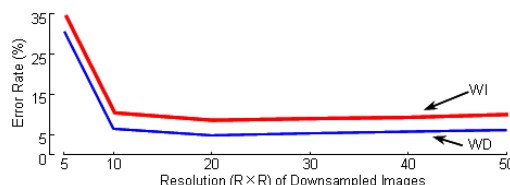
Figure 14. Error rate vs. Resolution. WD and WI tests on NicIcon dataset in 6 resolutions. Error rate makes little difference once the resolution is larger than 10×10.
