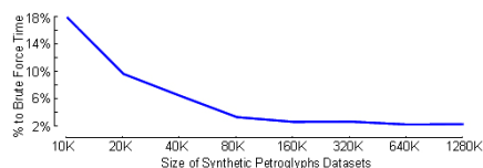
Figure 20. Percentage of execution time for our lower bound algorithm relative to the brute force algorithm. Note: log scale is used in x axis.
