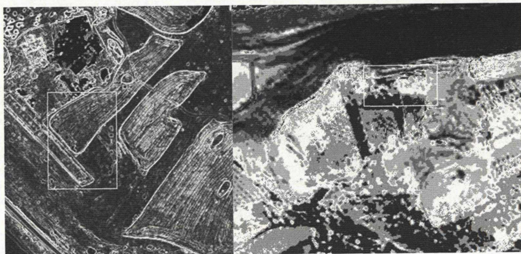
Figure 6 ISODATA classification using ATM11 and ATM12 with possible buried archaeological structures
