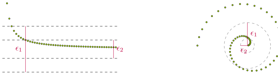
Figure 3.1: The illustration on the left shows the one-dimensional sequence \frac{1}{n} , where the ranges \epsilon_1 (resp. \epsilon_2 ) indicate the points that have distance \epsilon_1 (resp. \epsilon_2 ) to zero. The illustration on the right shows the sequence (x \cdot \cos(x), x \cdot \sin(x)) , which is Cauchy with respect to the usual metric on \mathbb{R}^2 .
